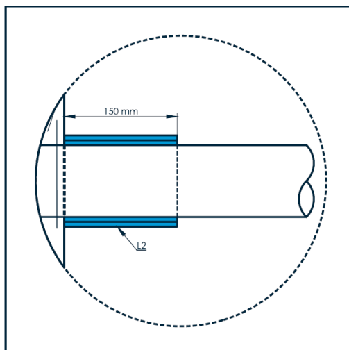
Figure 3 (3x150 mm) a: Minimum 10 mm overlap b: Mulcol Multitherm Bandage
