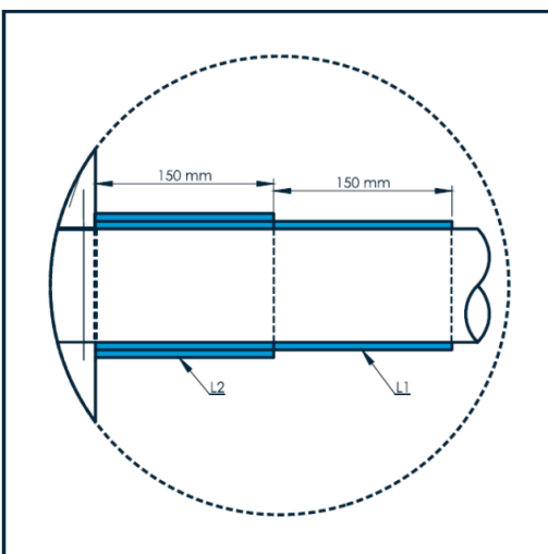
Figure 4 (2x150 mm + 1x150 mm) a: Minimum 10 mm overlap b: Mulcol Multitherm Bandage
