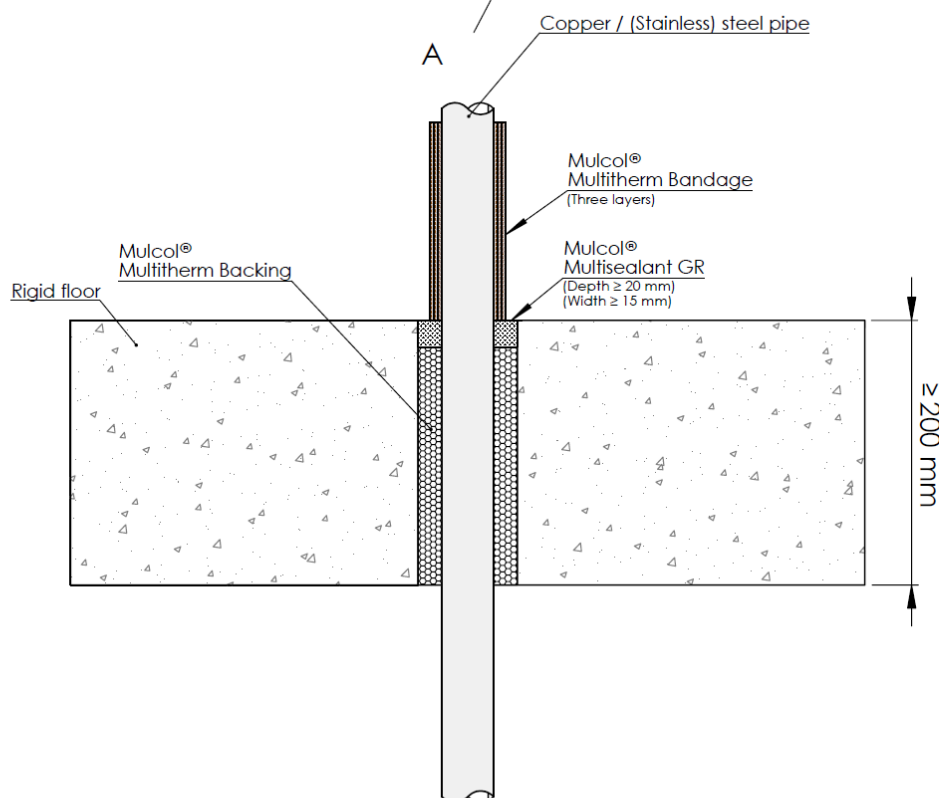
L3 - Three layers Mulcol® Multitherm Bandage
