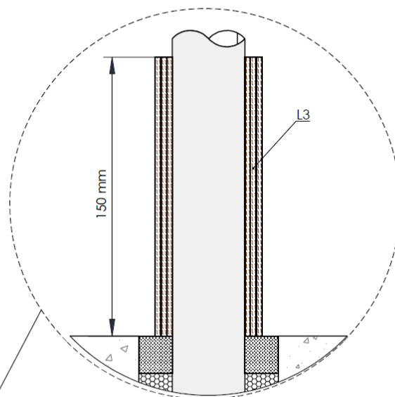
L3 - Three layers Mulcol® Multitherm Bandage
